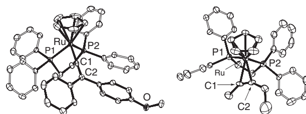
Figure 1. ORTEP drawings of 3a (left) and 4f (right). Anionic part and hydrogen atoms are omitted for clarity.
