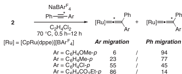
Scheme 4. Migratory aptitude of alkyne substituents. The asterisks represent 13 C-enriched carbon atoms.
